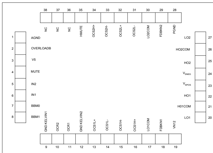
38 PIN QUAD MODULE PIN OUT TOP VIEW
